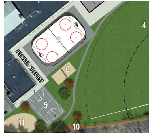
The Master Plan identifies a new court zone featuring full size basketball (5), beach volleyball (6), and skating rink (3). The open play field (outfield of the softball field) is shown to the right (4).
